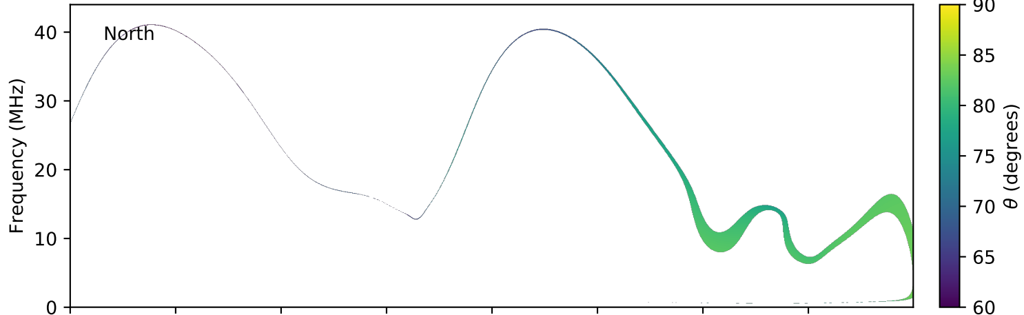
expres_earth_jupiter_europa_jrm09_lossc-wid1deg_3kev_20091106_v01.cdf
