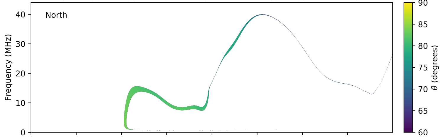
expres_earth_jupiter_europa_jrm09_lossc-wid1deg_3kev_20091105_v01.cdf
