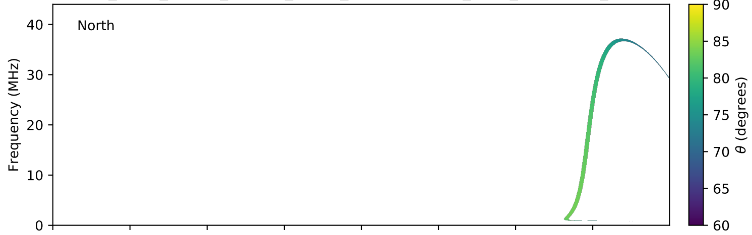
expres_earth_jupiter_europa_jrm09_lossc-wid1deg_3kev_20091101_v01.cdf
