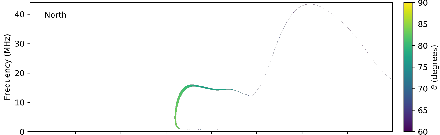
expres_earth_jupiter_io_jrm09_lossc-wid1deg_3kev_20091021_v01.cdf
