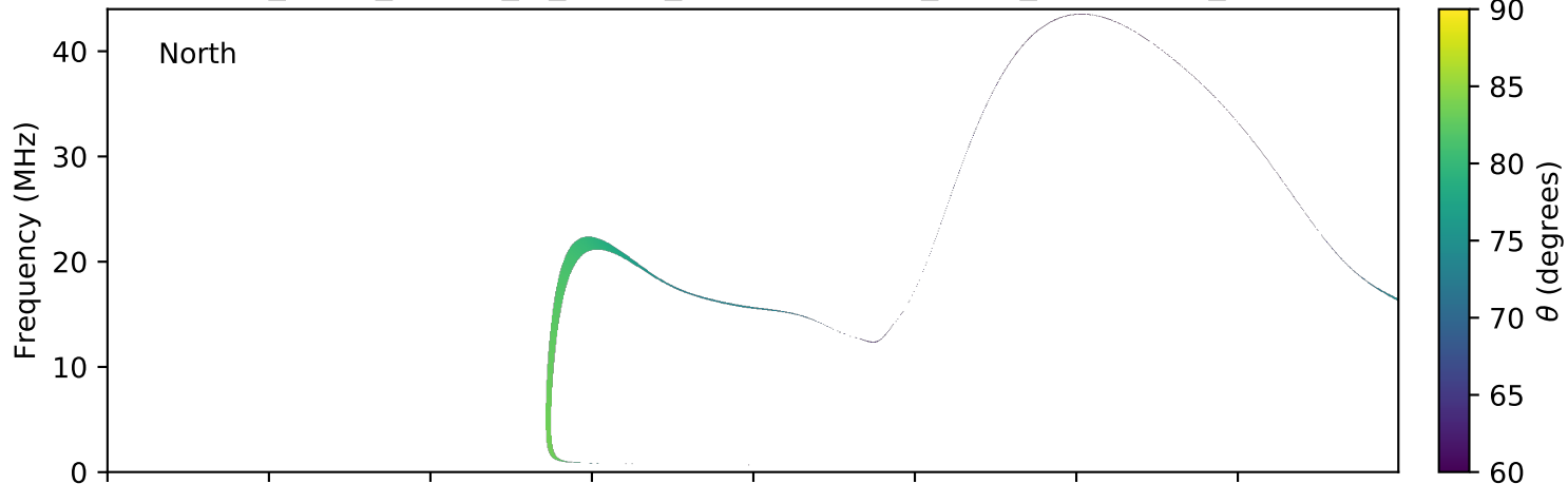
expres_earth_jupiter_io_jrm09_lossc-wid1deg_3kev_20091014_v01.cdf
