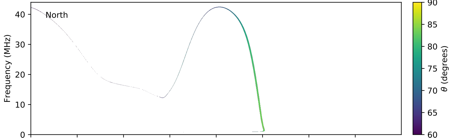
expres_earth_jupiter_io_jrm09_lossc-wid1deg_3kev_20091011_v01.cdf
