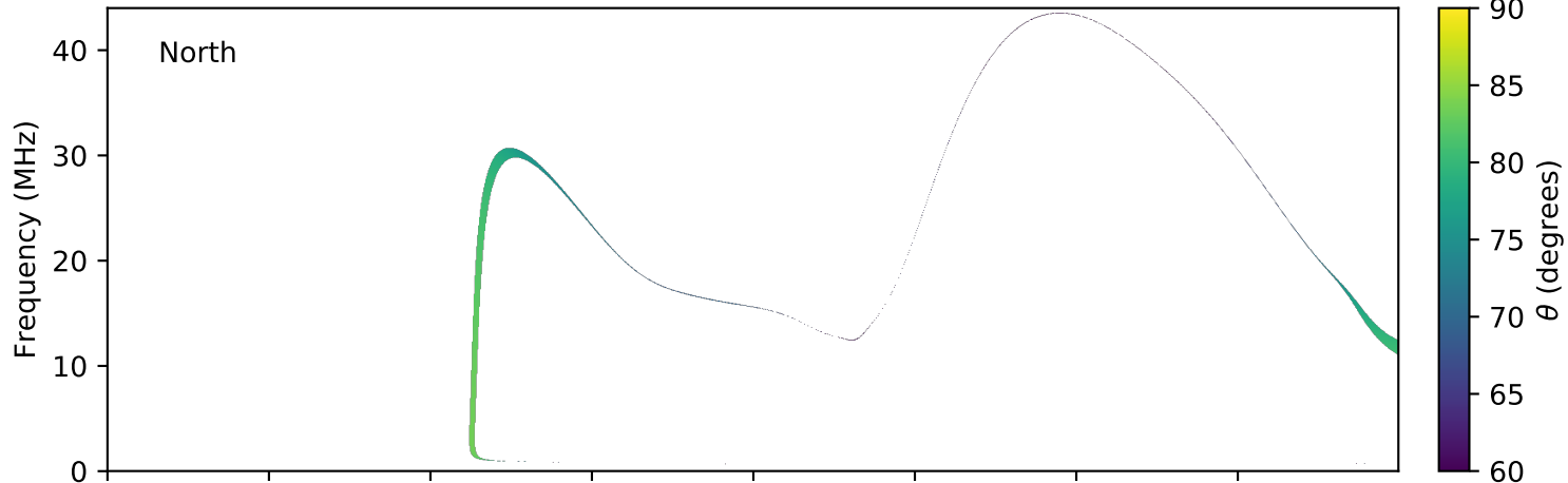
expres_earth_jupiter_io_jrm09_lossc-wid1deg_3kev_20091007_v01.cdf
