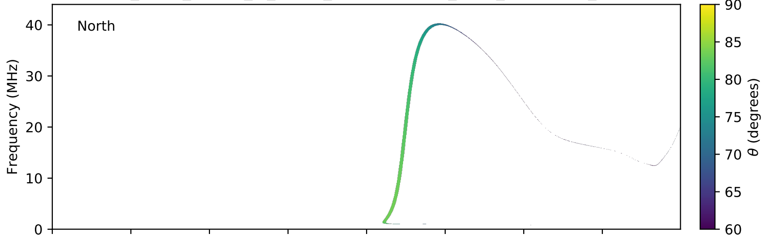
expres_earth_jupiter_io_jrm09_lossc-wid1deg_3kev_20091005_v01.cdf
