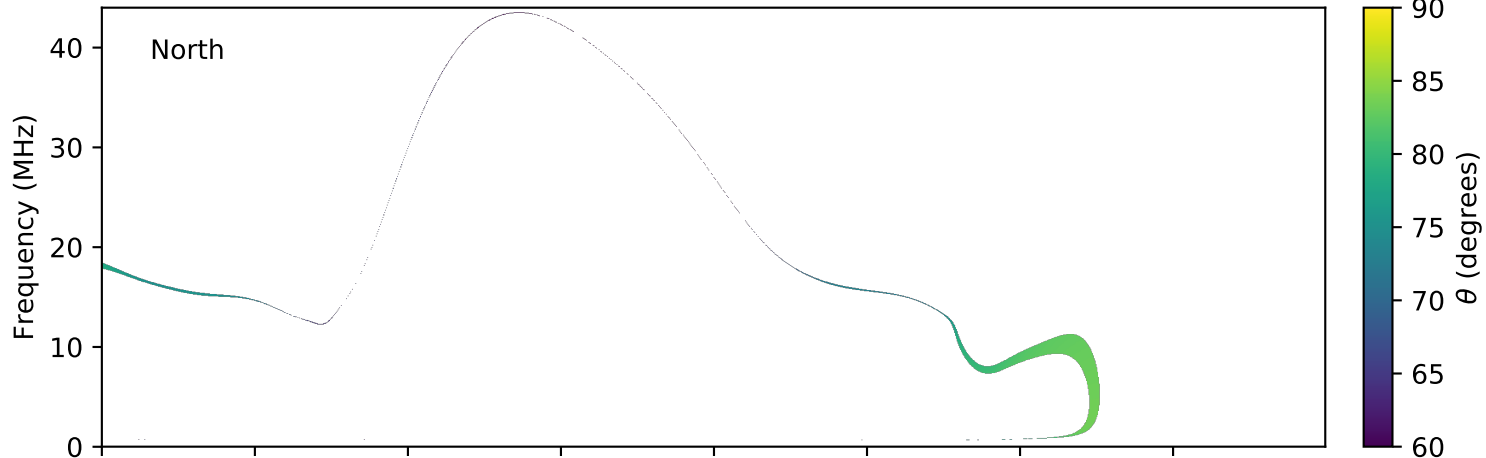
expres_earth_jupiter_io_jrm09_lossc-wid1deg_3kev_20091002_v01.cdf
