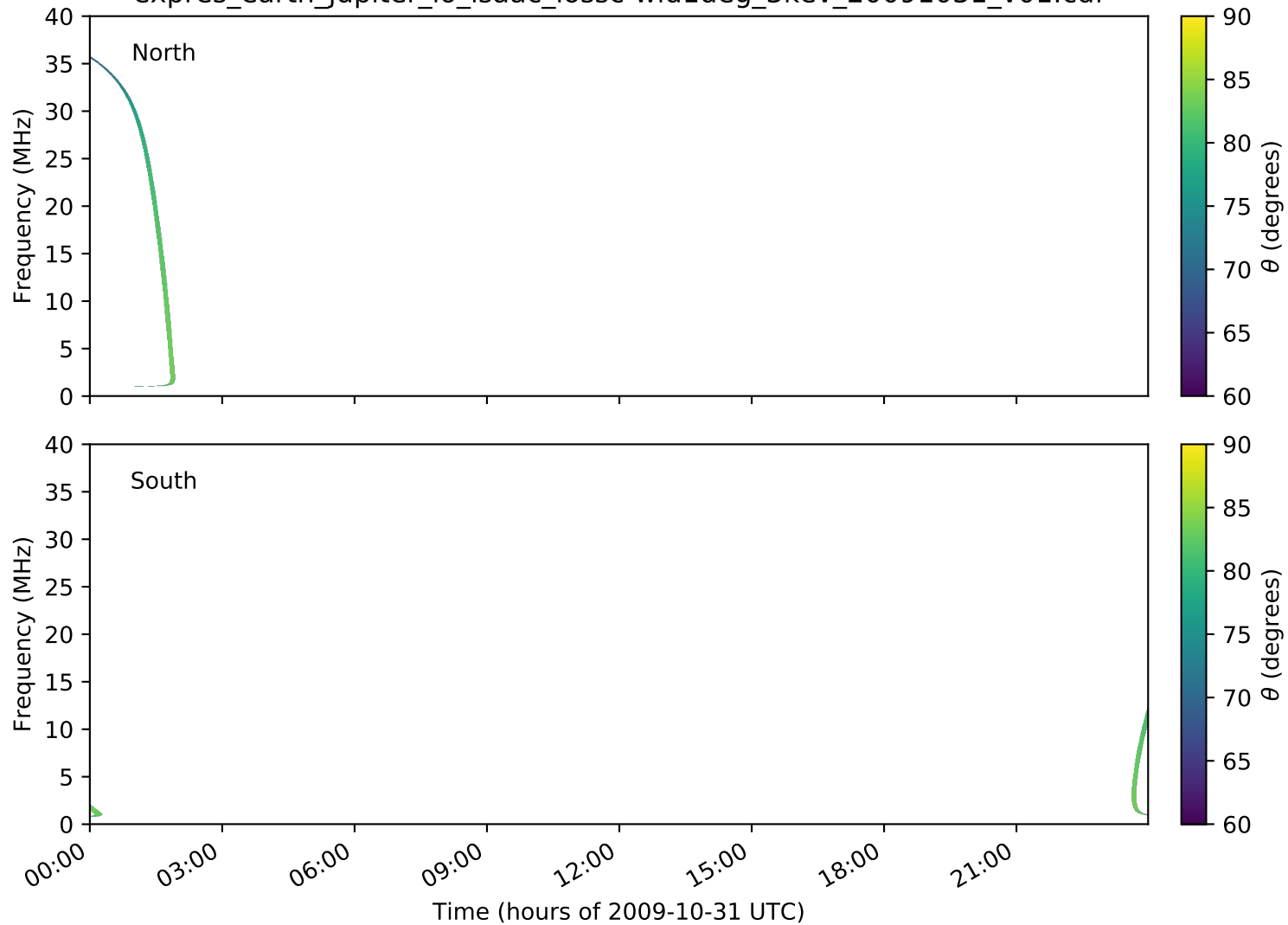
expres_earth_jupiter_io_isaac_lossc-wid1deg_3kev_20091031_v01.cdf
