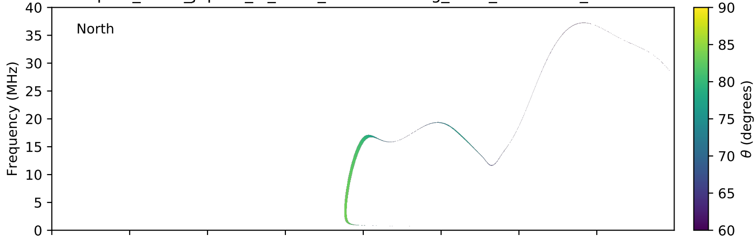
expres_earth_jupiter_io_isaac_lossc-wid1deg_3kev_20091028_v01.cdf
