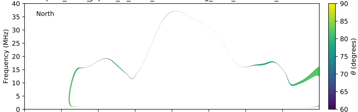
expres_earth_jupiter_io_isaac_lossc-wid1deg_3kev_20091023_v01.cdf
