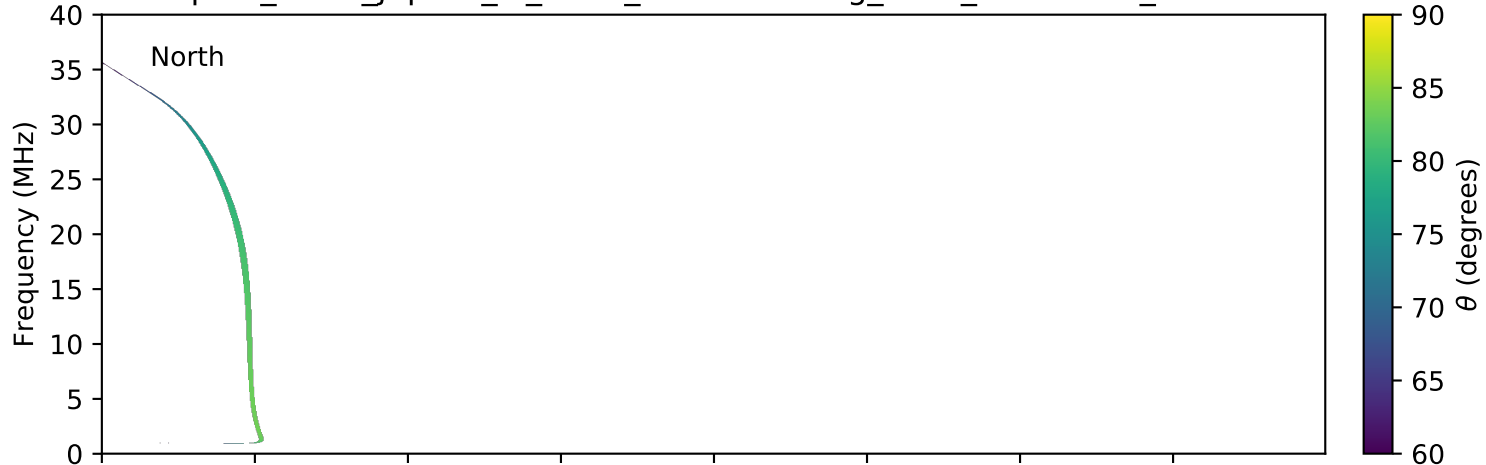
expres_earth_jupiter_io_isaac_lossc-wid1deg_3kev_20091015_v01.cdf
