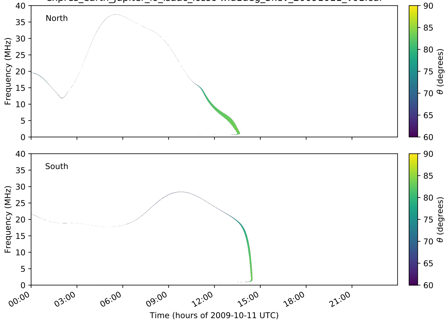
expres_earth_jupiter_io_isaac_lossc-wid1deg_3kev_20091011_v01.cdf
