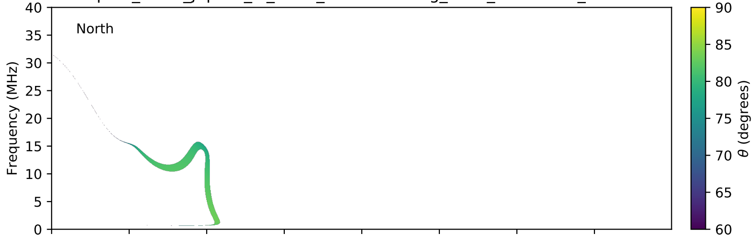
expres_earth_jupiter_io_isaac_lossc-wid1deg_3kev_20091006_v01.cdf
