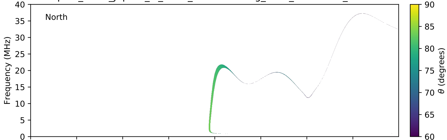
expres_earth_jupiter_io_isaac_lossc-wid1deg_3kev_20091005_v01.cdf
