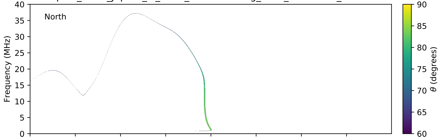
expres_earth_jupiter_io_isaac_lossc-wid1deg_3kev_20091004_v01.cdf
