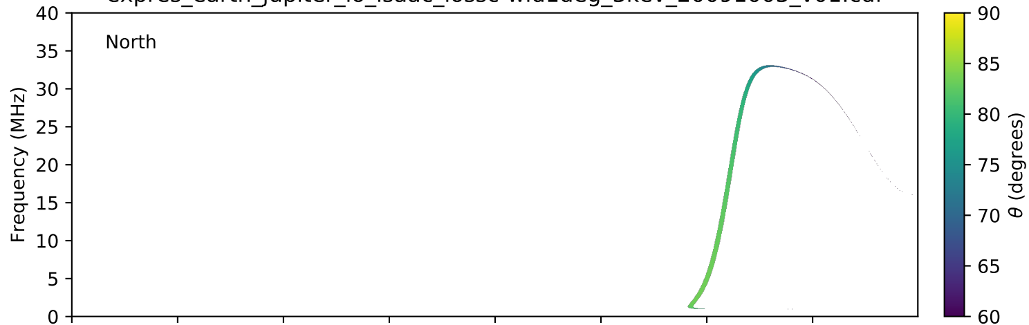
expres_earth_jupiter_io_isaac_lossc-wid1deg_3kev_20091003_v01.cdf
