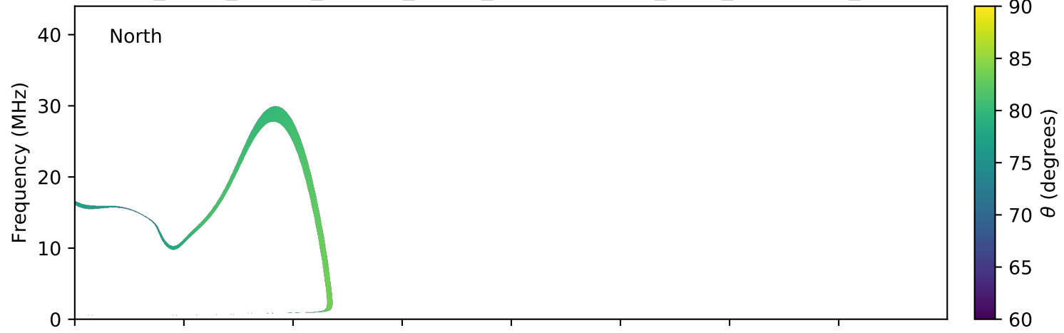
expres_earth_jupiter_europa_jrm09_lossc-wid1deg_3kev_20091027_v01.cdf
