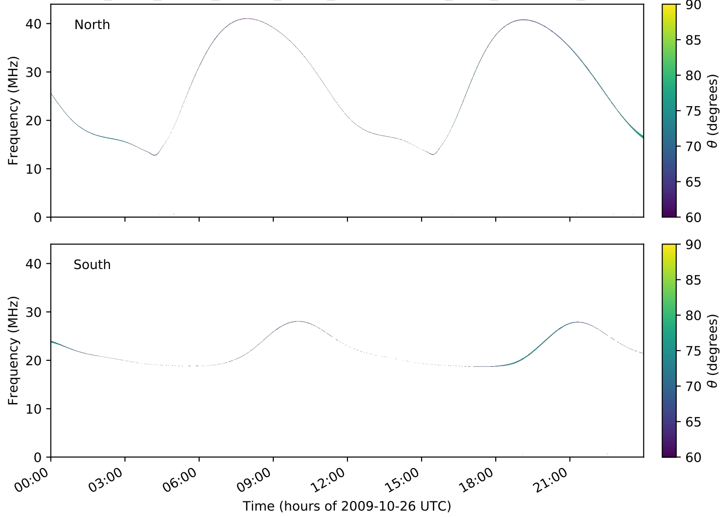
expres_earth_jupiter_europa_jrm09_lossc-wid1deg_3kev_20091026_v01.cdf
