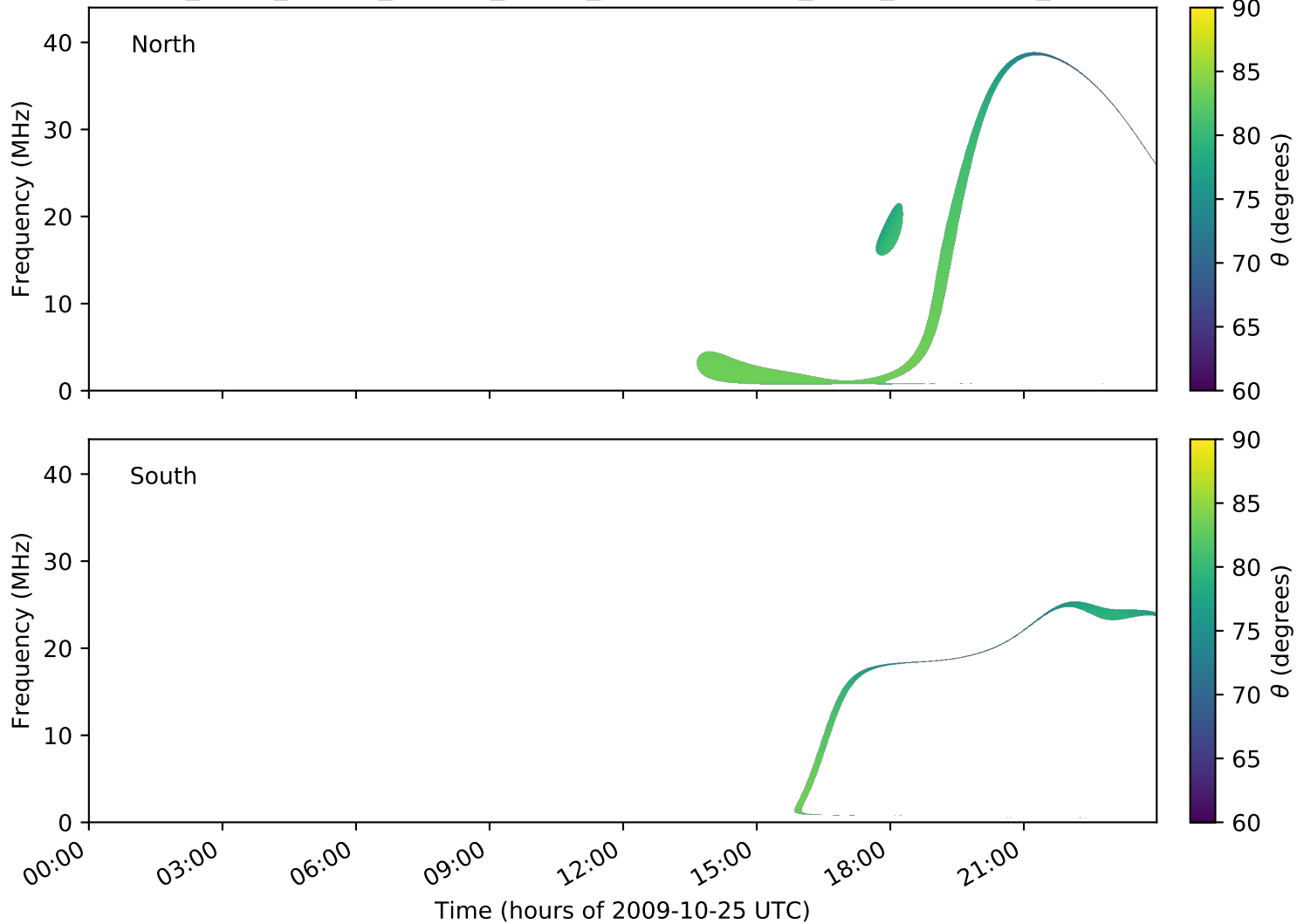
expres_earth_jupiter_europa_jrm09_lossc-wid1deg_3kev_20091025_v01.cdf
