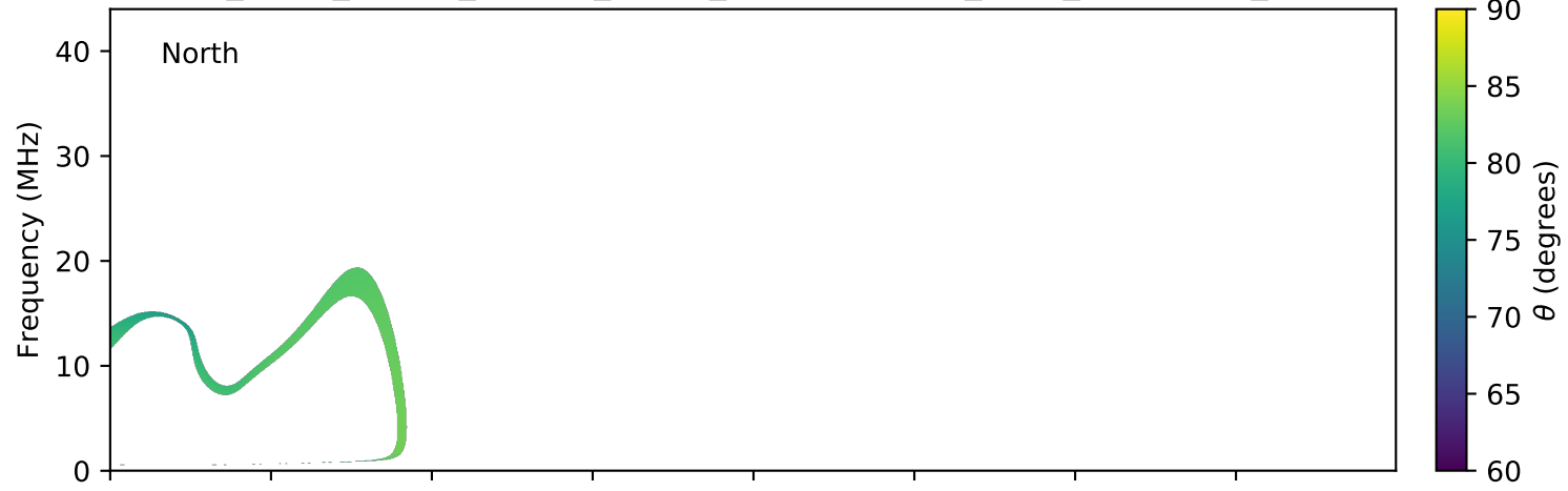
expres_earth_jupiter_europa_jrm09_lossc-wid1deg_3kev_20091020_v01.cdf
