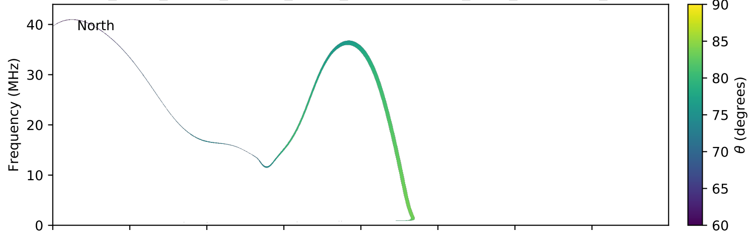
expres_earth_jupiter_europa_jrm09_lossc-wid1deg_3kev_20091016_v01.cdf
