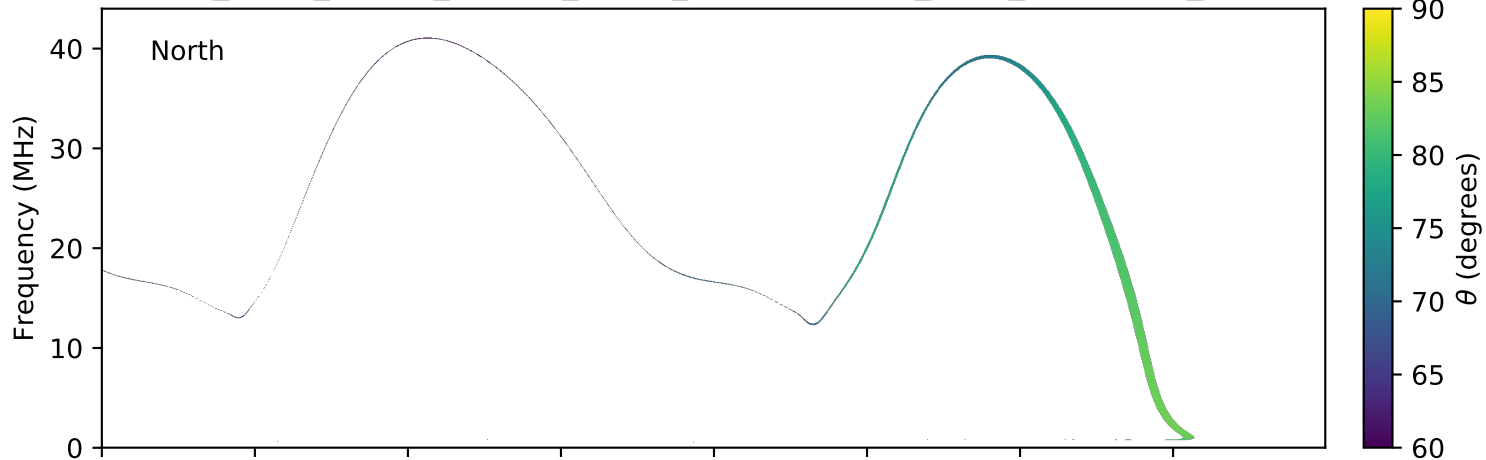
expres_earth_jupiter_europa_jrm09_lossc-wid1deg_3kev_20091005_v01.cdf
