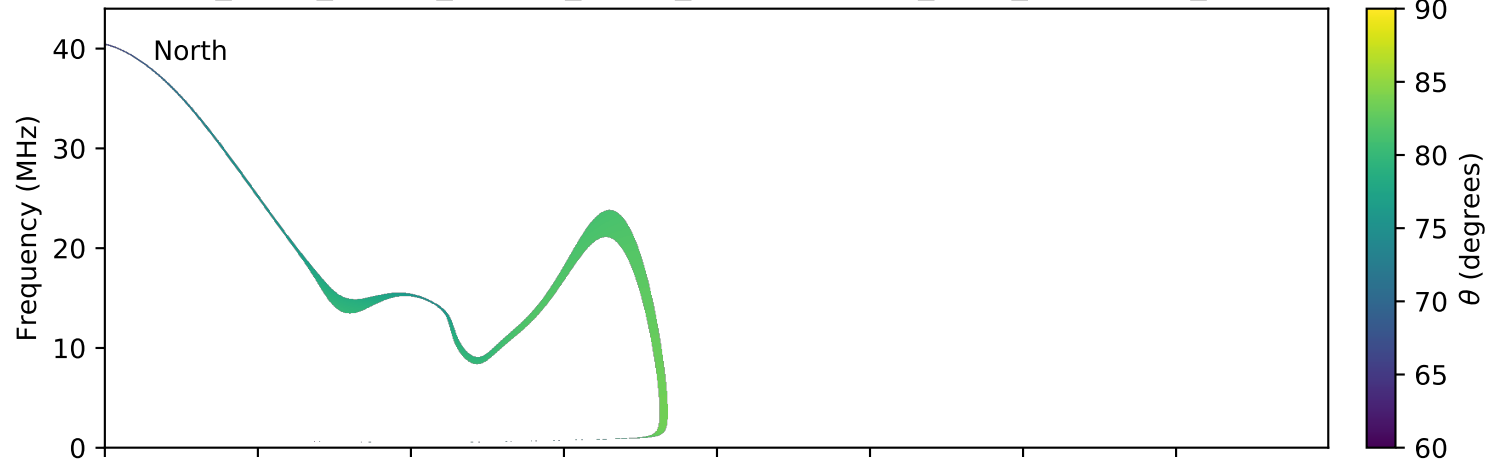
expres_earth_jupiter_europa_jrm09_lossc-wid1deg_3kev_20091002_v01.cdf
