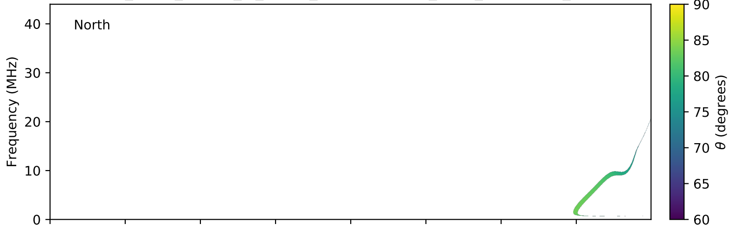
expres_earth_jupiter_io_jrm09_lossc-wid1deg_3kev_20090901_v01.cdf
