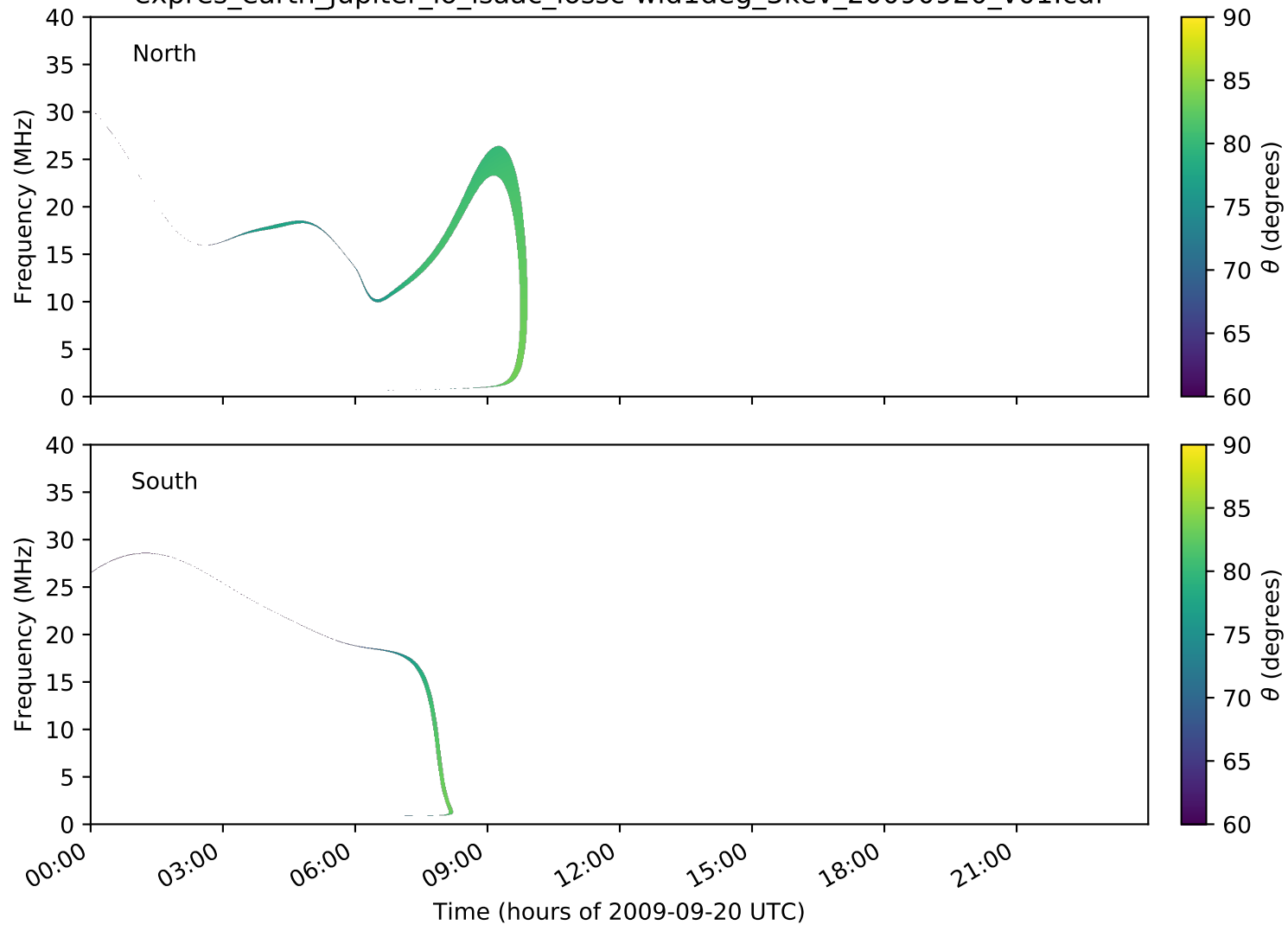
expres_earth_jupiter_io_isaac_lossc-wid1deg_3kev_20090920_v01.cdf
