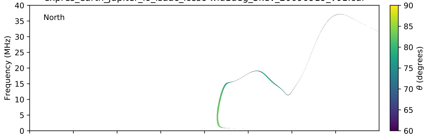
expres_earth_jupiter_io_isaac_lossc-wid1deg_3kev_20090919_v01.cdf
