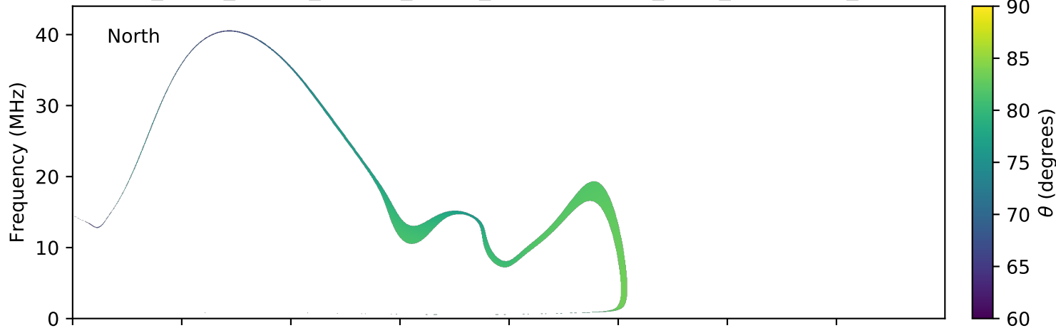
expres_earth_jupiter_europa_jrm09_lossc-wid1deg_3kev_20090907_v01.cdf
