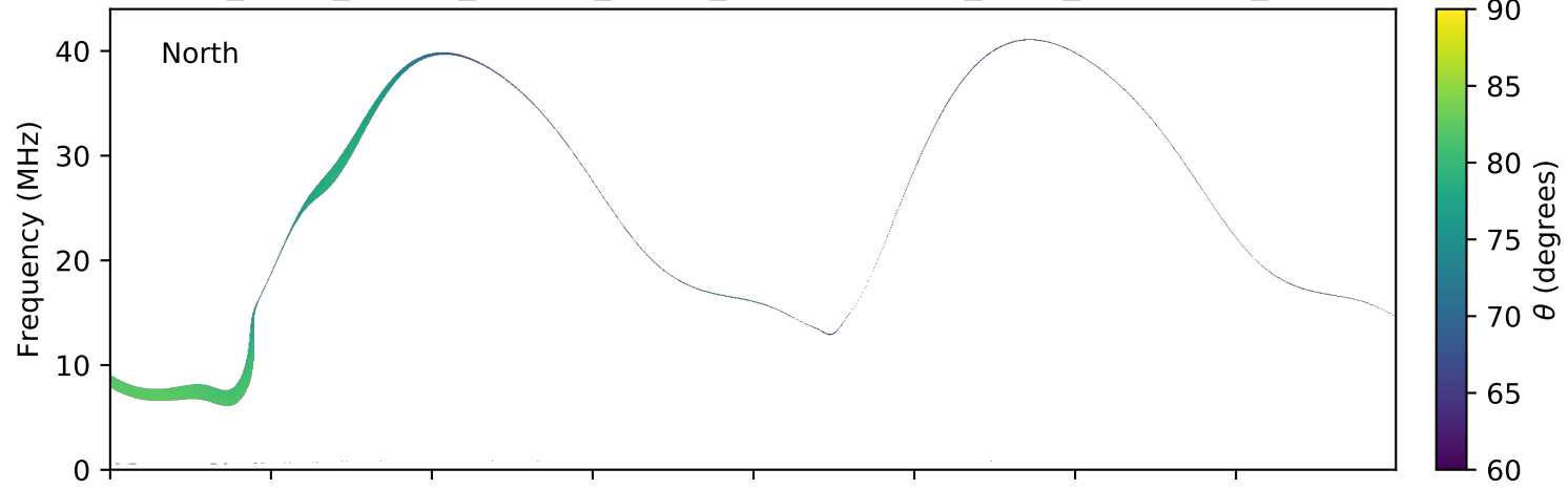
expres_earth_jupiter_europa_jrm09_lossc-wid1deg_3kev_20090906_v01.cdf
