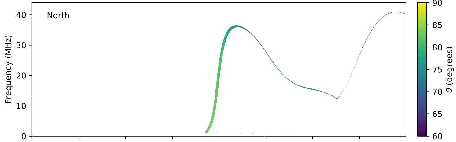
expres_earth_jupiter_europa_jrm09_lossc-wid1deg_3kev_20090902_v01.cdf
