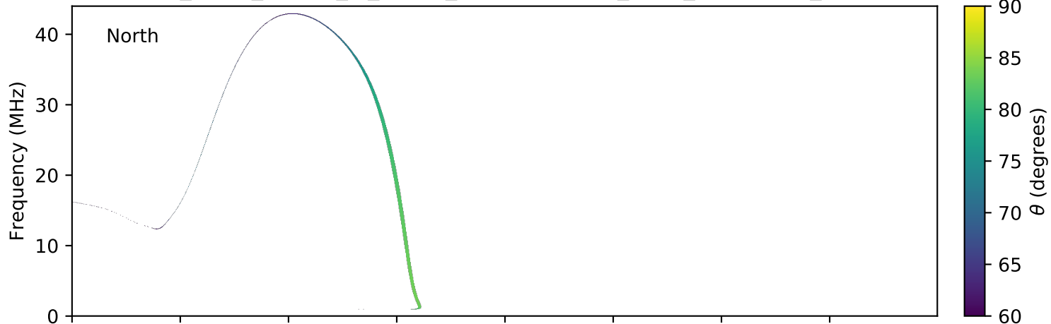
expres_earth_jupiter_io_jrm09_lossc-wid1deg_3kev_20090828_v01.cdf
