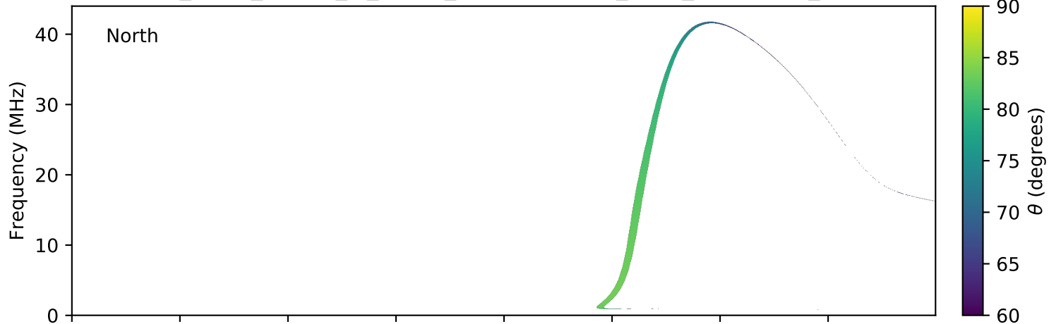
expres_earth_jupiter_io_jrm09_lossc-wid1deg_3kev_20090827_v01.cdf
