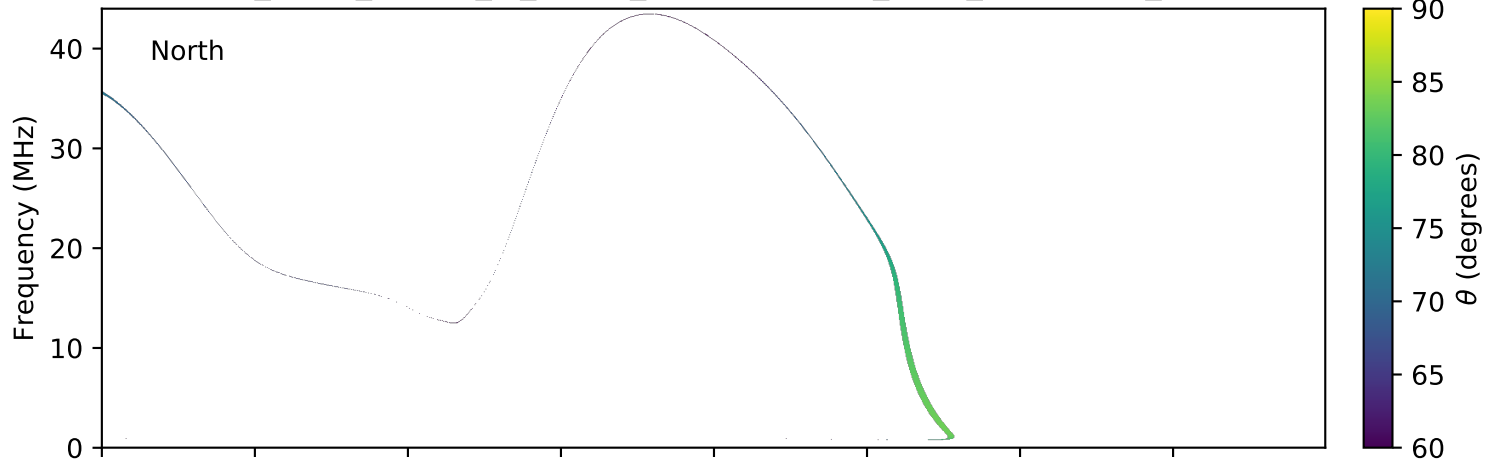
expres_earth_jupiter_io_jrm09_lossc-wid1deg_3kev_20090810_v01.cdf
