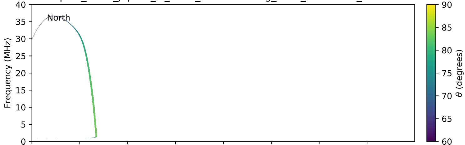
expres_earth_jupiter_io_isaac_lossc-wid1deg_3kev_20090830_v01.cdf
