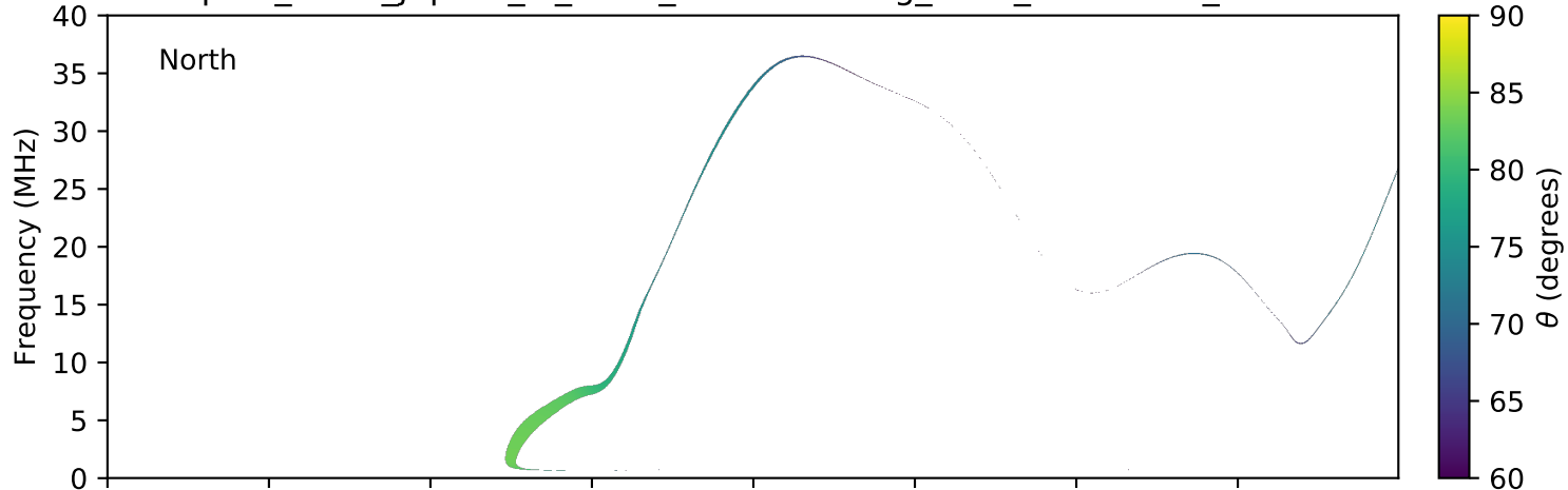
expres_earth_jupiter_io_isaac_lossc-wid1deg_3kev_20090829_v01.cdf
