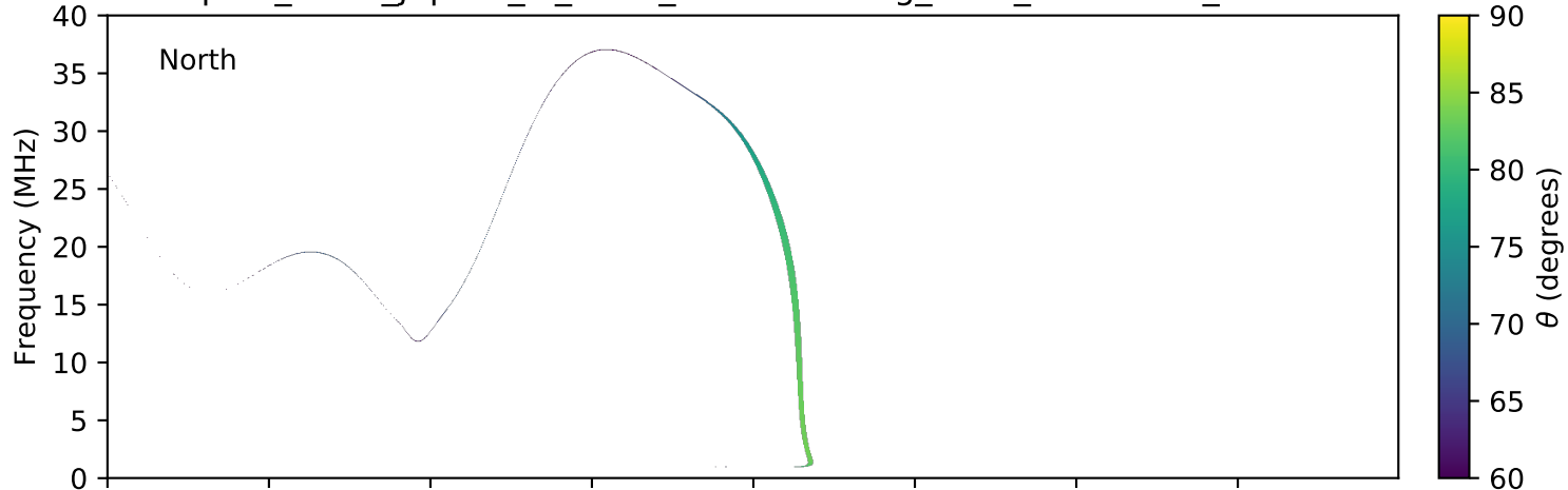
expres_earth_jupiter_io_isaac_lossc-wid1deg_3kev_20090819_v01.cdf
