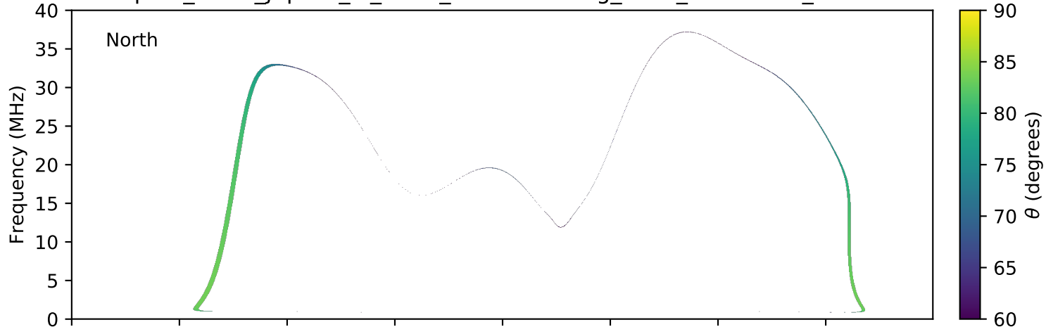
expres_earth_jupiter_io_isaac_lossc-wid1deg_3kev_20090808_v01.cdf
