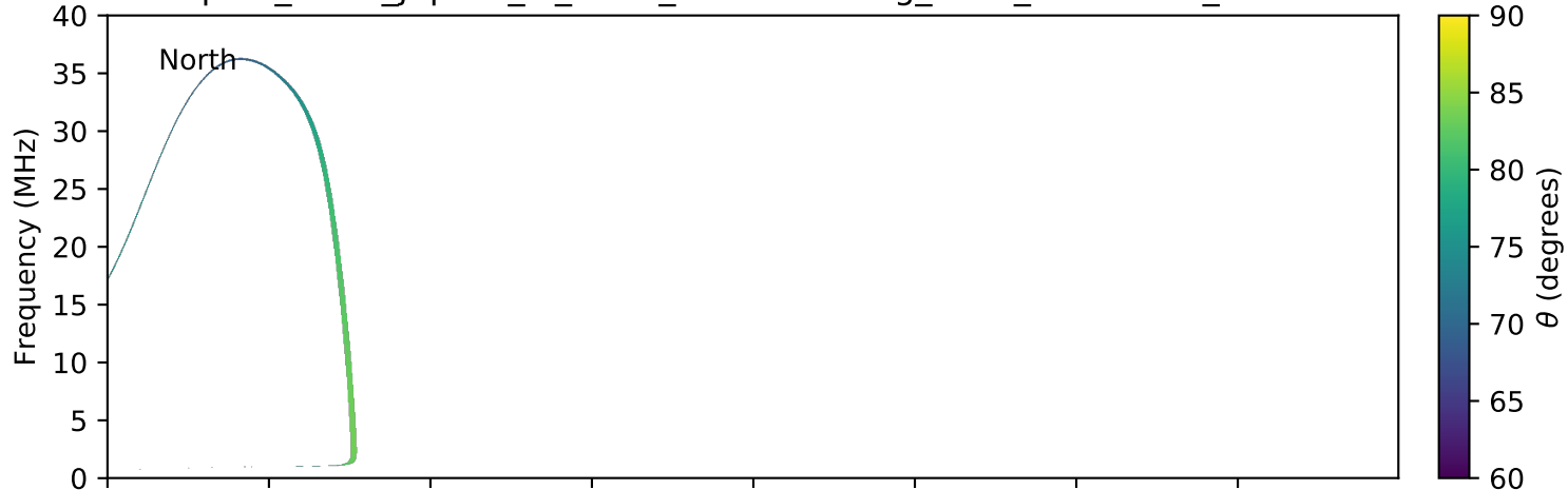
expres_earth_jupiter_io_isaac_lossc-wid1deg_3kev_20090807_v01.cdf
