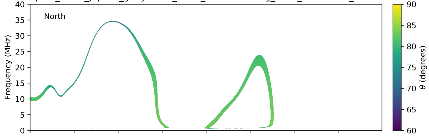
expres_earth_jupiter_ganymede_isaac_lossc-wid1deg_3kev_20090821_v01.cdf
