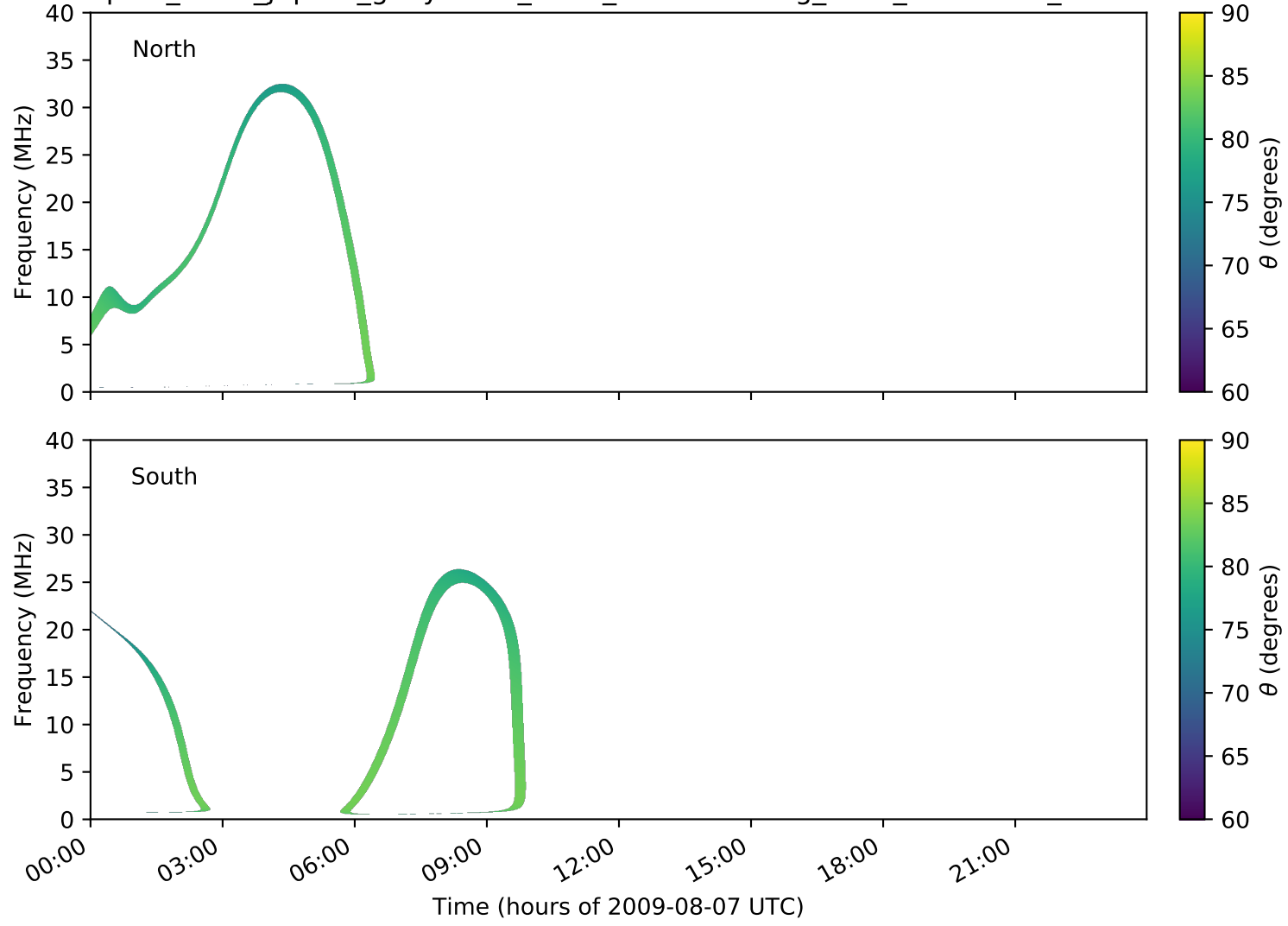
expres_earth_jupiter_ganymede_isaac_lossc-wid1deg_3kev_20090807_v01.cdf
