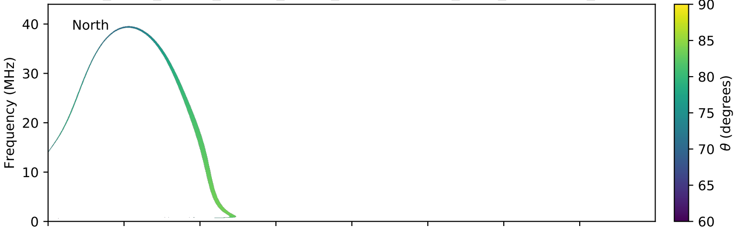
expres_earth_jupiter_europa_jrm09_lossc-wid1deg_3kev_20090824_v01.cdf
