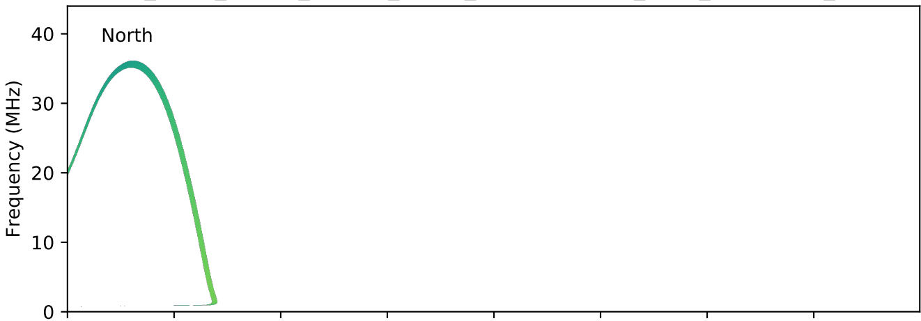
expres_earth_jupiter_europa_jrm09_lossc-wid1deg_3kev_20090810_v01.cdf
