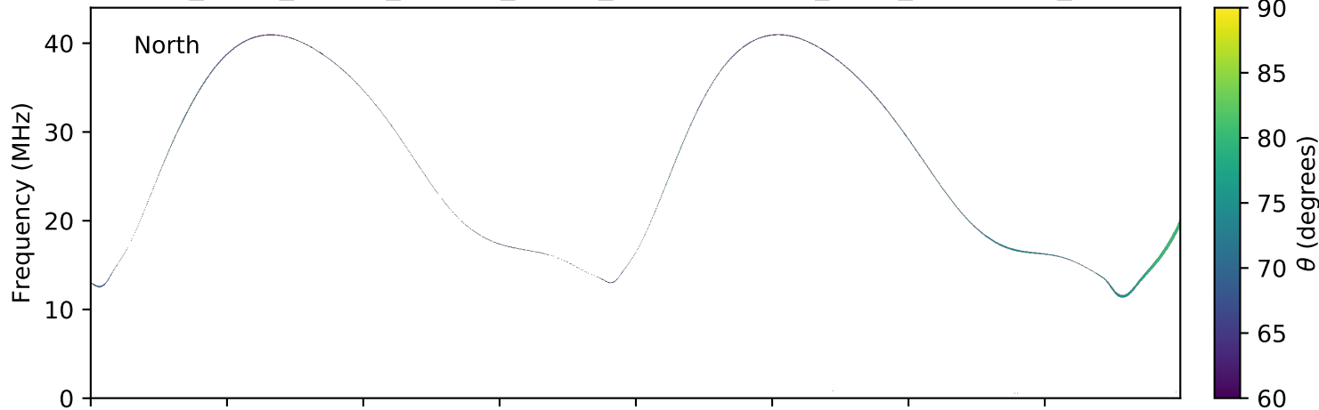
expres_earth_jupiter_europa_jrm09_lossc-wid1deg_3kev_20090809_v01.cdf
