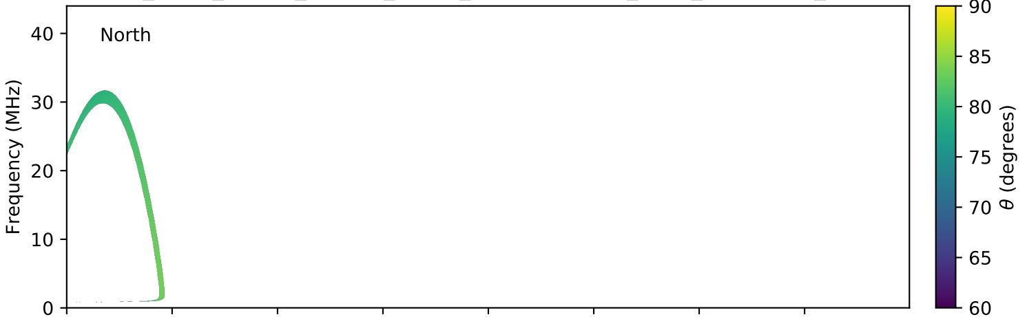
expres_earth_jupiter_europa_jrm09_lossc-wid1deg_3kev_20090803_v01.cdf
