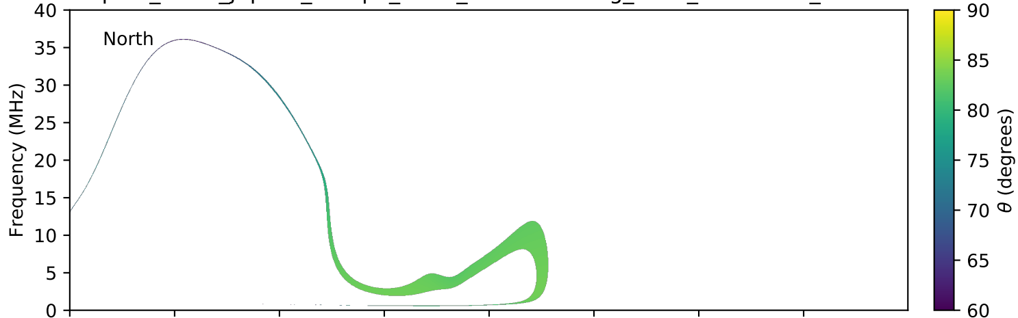
expres_earth_jupiter_europa_isaac_lossc-wid1deg_3kev_20090831_v01.cdf
