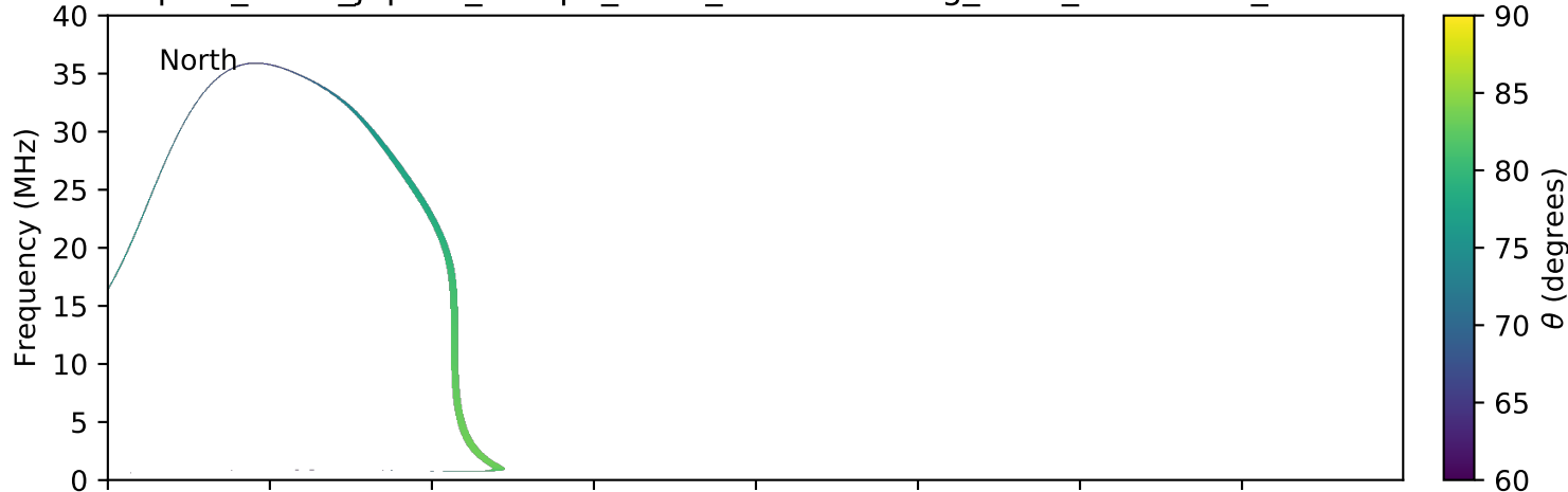
expres_earth_jupiter_europa_isaac_lossc-wid1deg_3kev_20090824_v01.cdf
