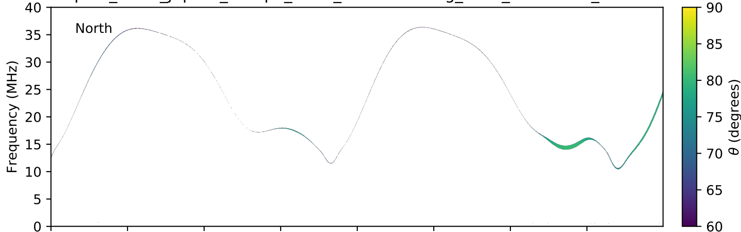
expres_earth_jupiter_europa_isaac_lossc-wid1deg_3kev_20090809_v01.cdf
