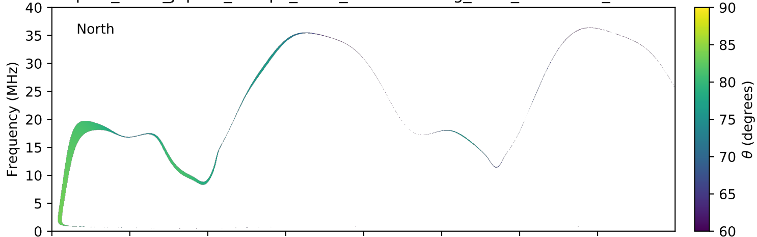
expres_earth_jupiter_europa_isaac_lossc-wid1deg_3kev_20090805_v01.cdf
