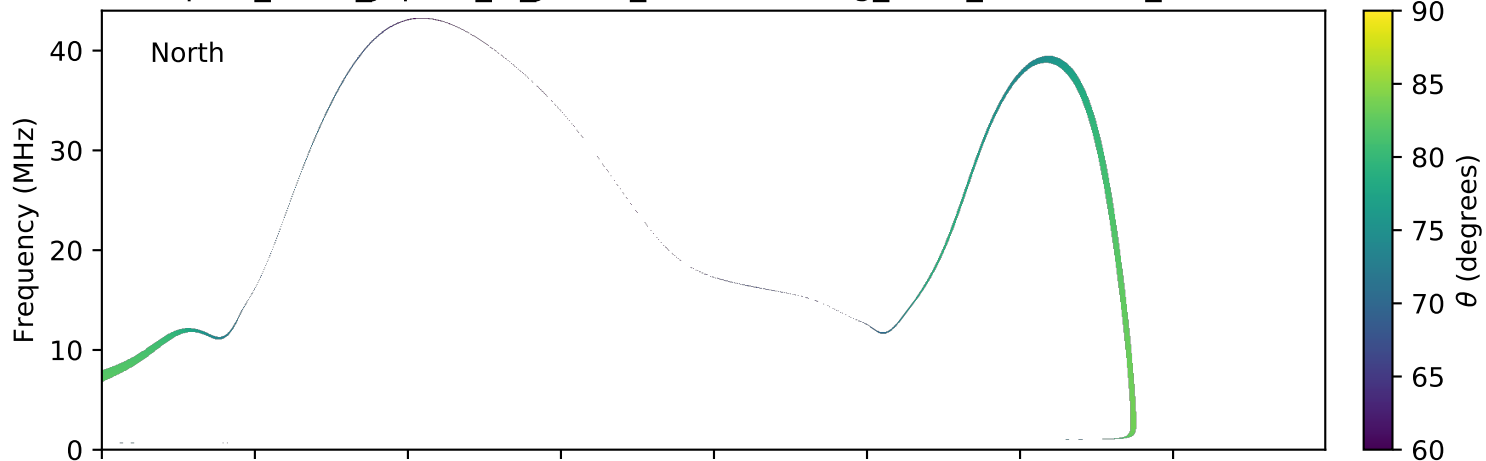
expres_earth_jupiter_io_jrm09_lossc-wid1deg_3kev_20090725_v01.cdf
